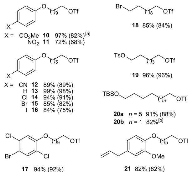
Scheme 3. Two-step deoxygenation of 1° alcohols by the Cu-catalyzed reduction of 1° alkyl triflates. Yields of isolated products are shown; overall yields for the two-step triflation/reduction sequence are given in parentheses. [a] 1 mol % of catalyst was used. [b] Reaction was performed on a 20 mmol scale and yielded 3.6 g of the product.
