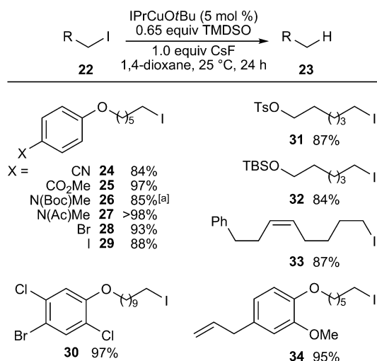
Scheme 4. Cu-catalyzed reduction of 1° alkyl iodides. Yields of isolated products are shown. [a] 1.4 equiv Ph 2 SiH 2 and 1.1 equiv 37 were used instead of TMSO and CsF. Ac = acetyl, Boc = tert -butoxycarbonyl.
